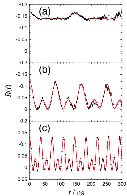
Fig. 1. TDPAC spectra of 111 Cd( \leftarrow 111 In) in Fe 3 O 4 (a) at 900 K, (b) at 773 K, and (c) at R. T.
