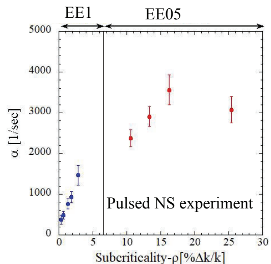
Fig.4. Prompt-neutron decay constant \alpha determined from pulsed neutron source experiment.
