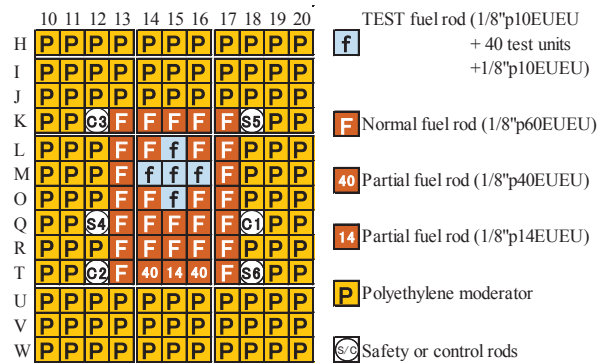
Figure 1. Reference core configuration
