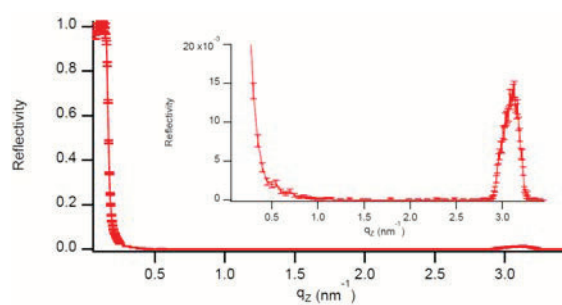
Fig. 2. Measured reflectivity of neutrons by d ~2nm multilayer mirror fabricated on center position (U0) shown in Fig.1. The inserted figure is a figure with the maximum of the vertical axis set to 2%. The effective number of layers of the multilayer mirrors is 1680.
