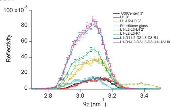
Fig. 3. Measured reflectivity of neutrons by stacking d ~2nm multilayer mirrors fabricated on various positions shown in Fig.1.
