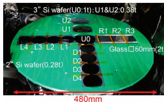
Fig. 1. The photograph of substrate arrangement on a substrate holder of KUR-IBS.
