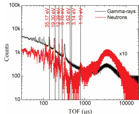
Fig. 2. TOF spectra obtained by the NRFNA experiment.
