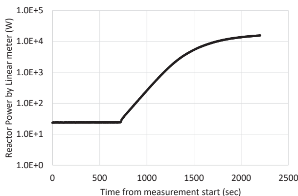
Fig. 2. Reactor power.
