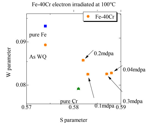
Fig. 2. Changess of S and W parameters with dose of electron irradiation of Fe-40Cr alloy in comparison with unirradiated pure Fe, pure Cr and Fe-40Cr alloy (As WQ).
