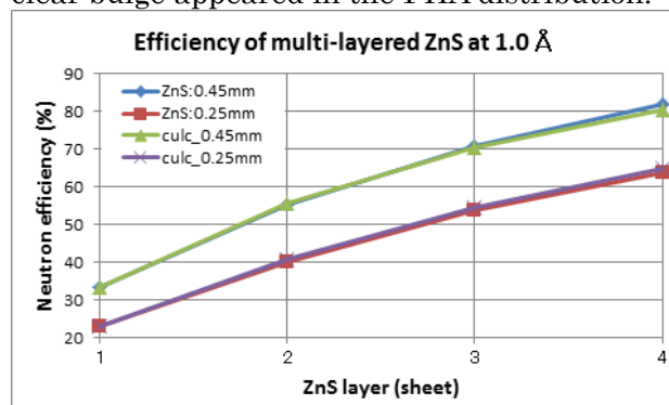
Fig. 1. Neutron detection efficiency of multi-layered ZnS scintillator.
