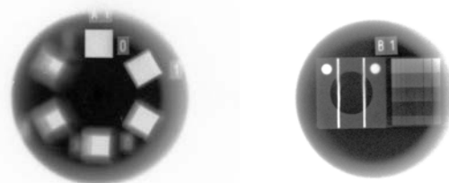
Fig.2 Results of neutron imaging by Dy foil transfer method (left: Gd 2 O 3 S ceramic plates, right: Indicators)
