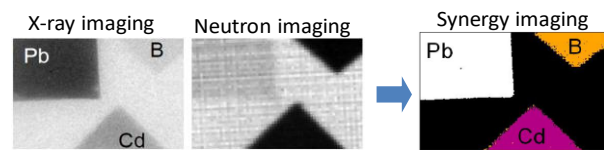
Fig.2. Synergy imaging for 2D-sample.
