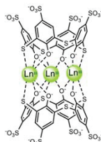
Fig. 1 Structure of \text{Ln}_3\text{TCAS}_2 complex.
